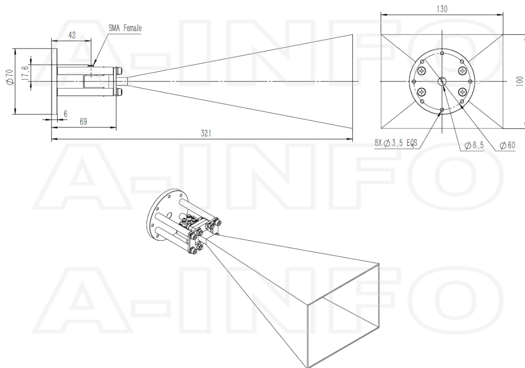
SMA-Female Output with Round Mounting Bracket (Option, P/N: LB-51-10-C-MB)
