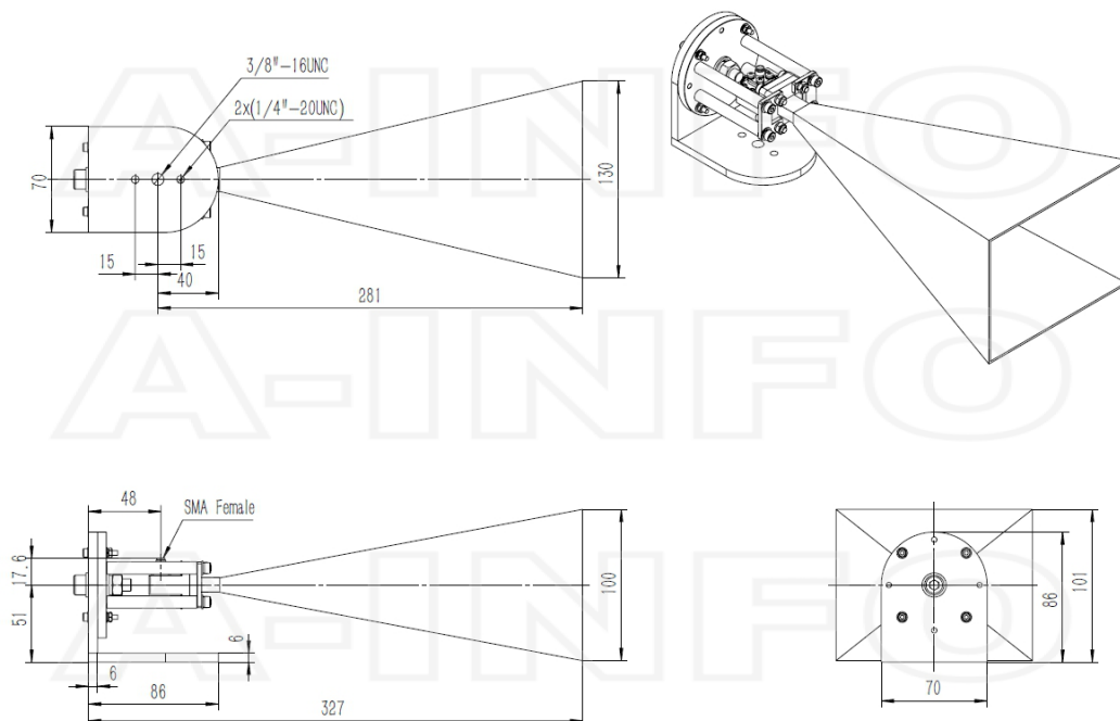
SMA-Female Output with L Type Mounting Bracket (Option, P/N: LB-51-10-C-MBL)
